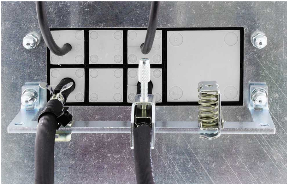
Illustration: EMC rails for the KDSClick cable entry system enable safe and secure shield connection
